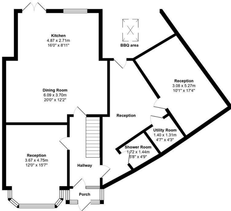
Ground Floor Area: 100.8 m 2 ... 1085 ft 2
